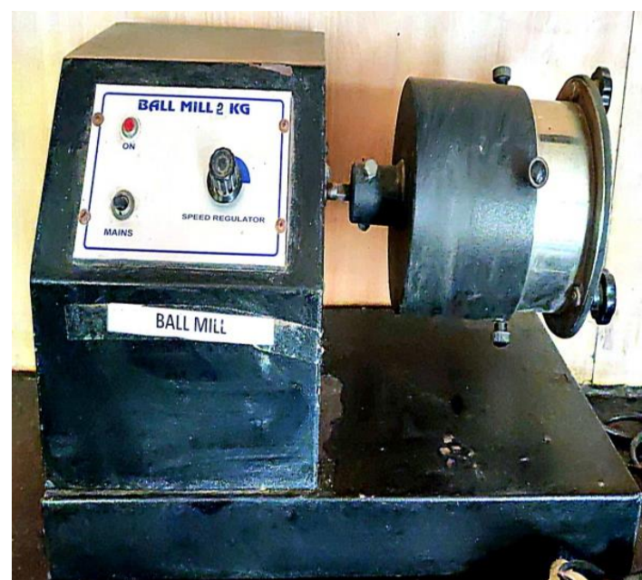
BALL MILL
